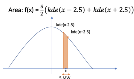
Figure 14 : Once a kernel density estimator is built, the trapezoidal method is used to store the distribution of each value between -2500 and +2500 MW with a step of 5 MW.
